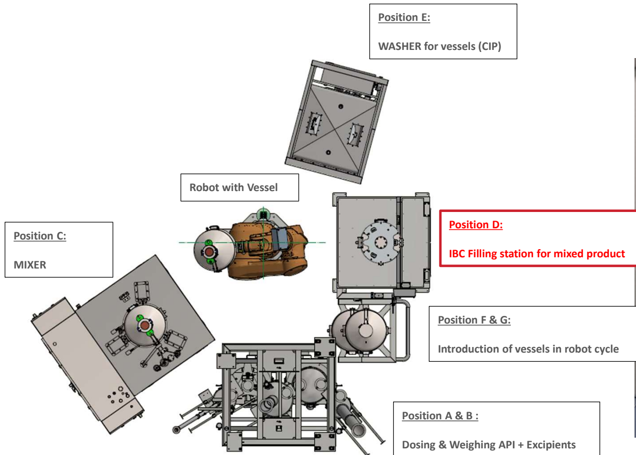
Filling of finished product into IBC
