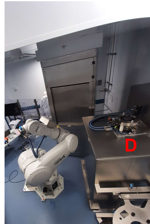
Filling of finished product into IBC
